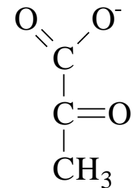
Pyruvate
