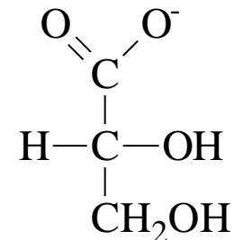
Glycerate
