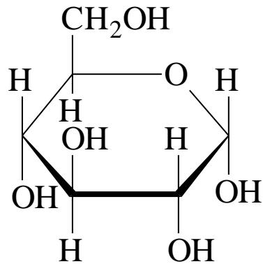
Glucose
