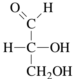
Glyceraldehyde
